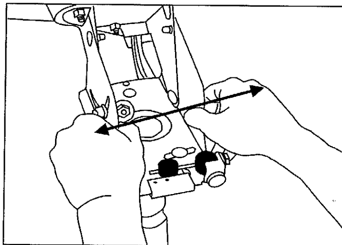
When moving the Dish to the Left and Right Dither stops, grasp the rear of the mount, not the Dish
