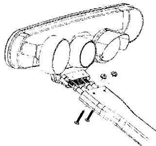
Hooking up cables to the LNB and attaching the LNB to Antenna — up to four cables can be connected this way.
