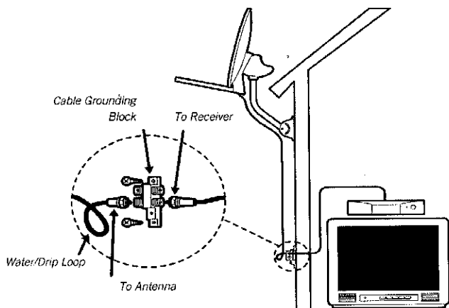
Dual grounding block, one receiver hook up shown
