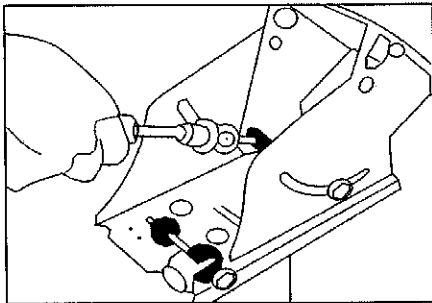
Use a 1/2" Nut Driver to turn the Elevation Fine-tune screw. Accurately count turns during this step
