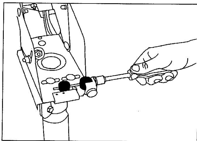
Use a 1/2" Nut Driver to adjust the Azimuth Fine-tune until the exact same signal level is reached at the Left and Right Dither stops
