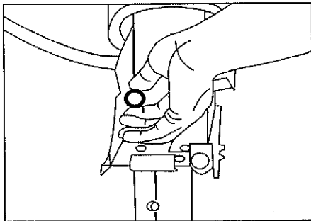
Start Elevation Fine-tune by grasping the black Elevation readout dial and rotate until "0" is lined up with the indicator
