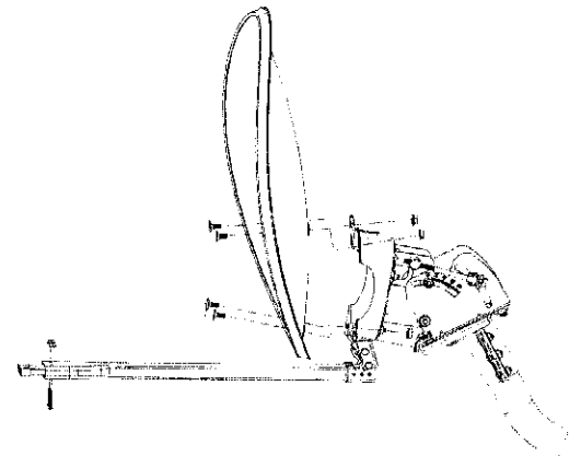
Dish Assembly with AZ/EL Back Assembly Type 2, WNC# BAU
