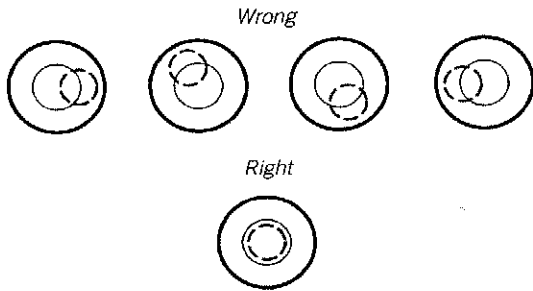
View of bubble level on top of mast
