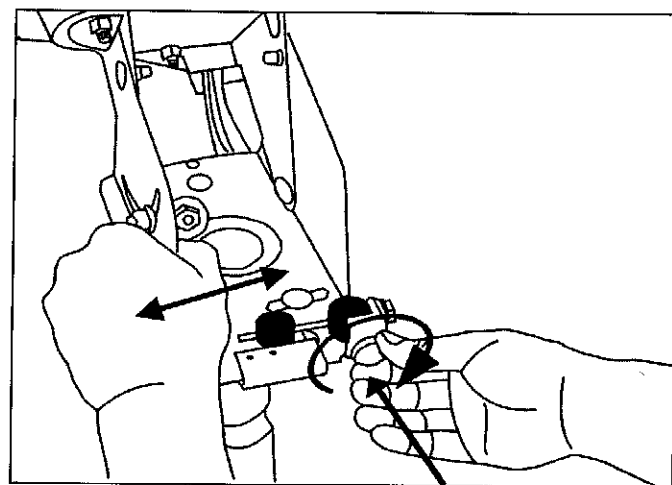
When replacing the Dither Pin, center the mount and rock side-to-side while rotating the Dither Pin Clockwise.
